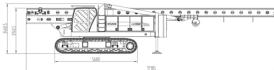
LH85 transport dimensions with folded leader configuration (Without Hydraulic Impact Hammer HHP8).
