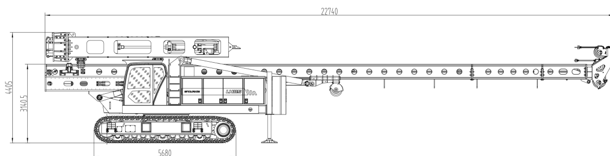
LH85 transport dimensions with standard leader configuration (Hydraulic Impact Hammer HHP8).
