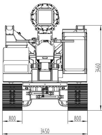
Minimum track width.
